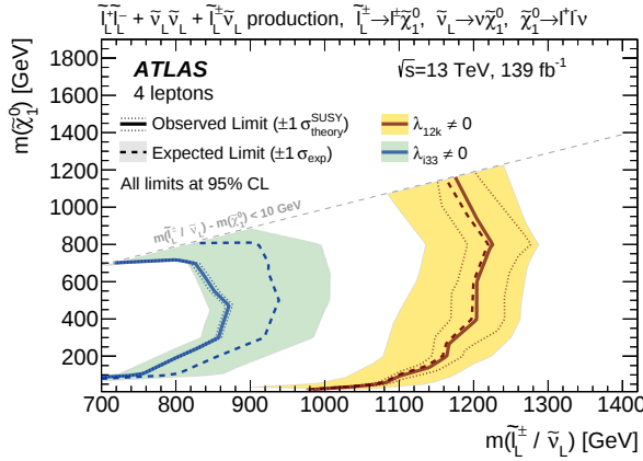
(c) RPV \tilde{\chi}_L / \tilde{\nu} NLSP
