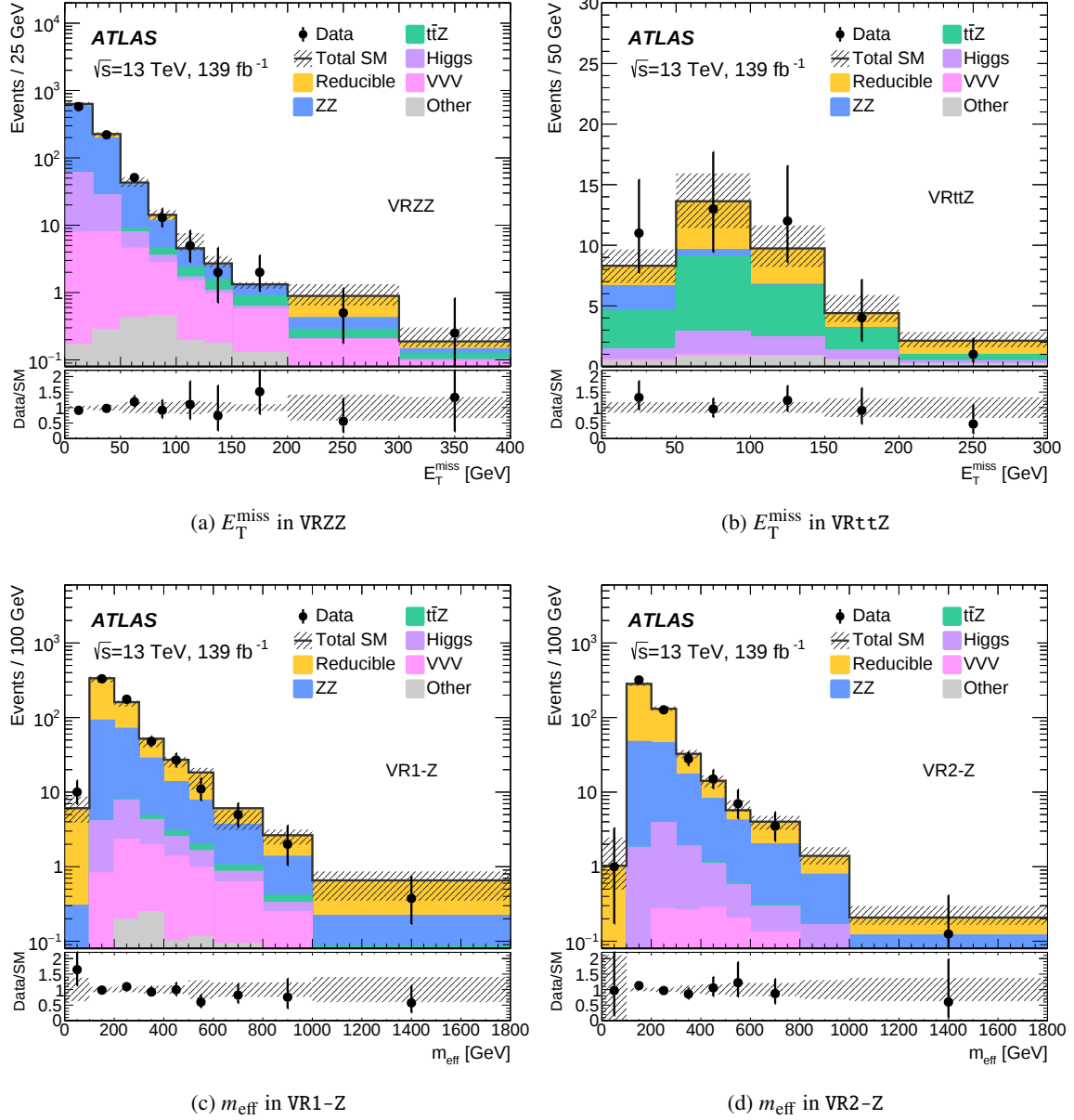
Figure 5: The distributions for data and the estimated SM backgrounds in the validation regions after the background-only fit, for the E_T^{\text{miss}} in (a) VRZZ and (b) VRttZ, and the m_{\text{eff}} in (c) VR1-Z and in (d) VR2-Z. “Other” is the sum of the tWZ , t\bar{t}WW , t\bar{t}ZZ , t\bar{t}WH , t\bar{t}HH , t\bar{t}tW , and t\bar{t}t\bar{t} backgrounds. The last bin includes the overflow. The lower panel shows the ratio of the observed data to the expected SM background yield in each bin. Both the statistical and systematic uncertainties in the SM background are included in the shaded band.
